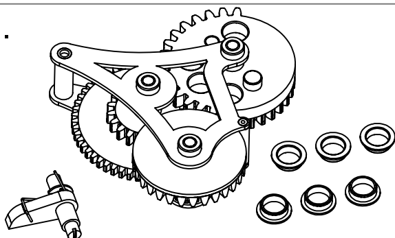
Modular Gear Set
